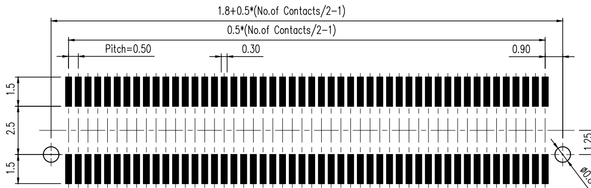
PCB Layout For Surface Mounting
